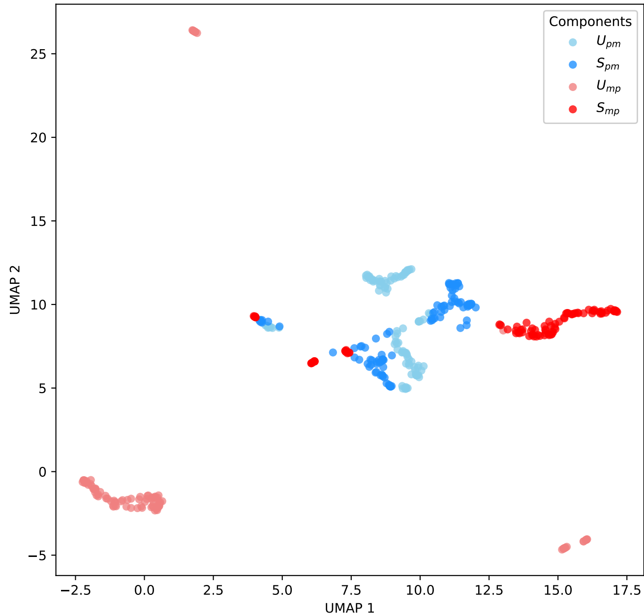
TCGA-PRAD: path vs mol
