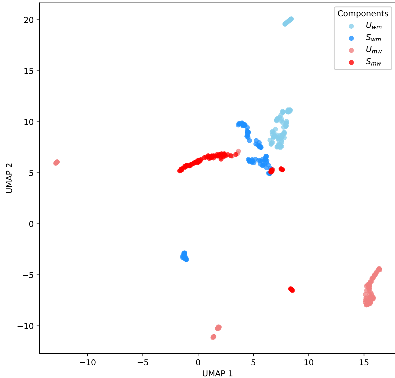
TCGA-PRAD: wsi vs mol
