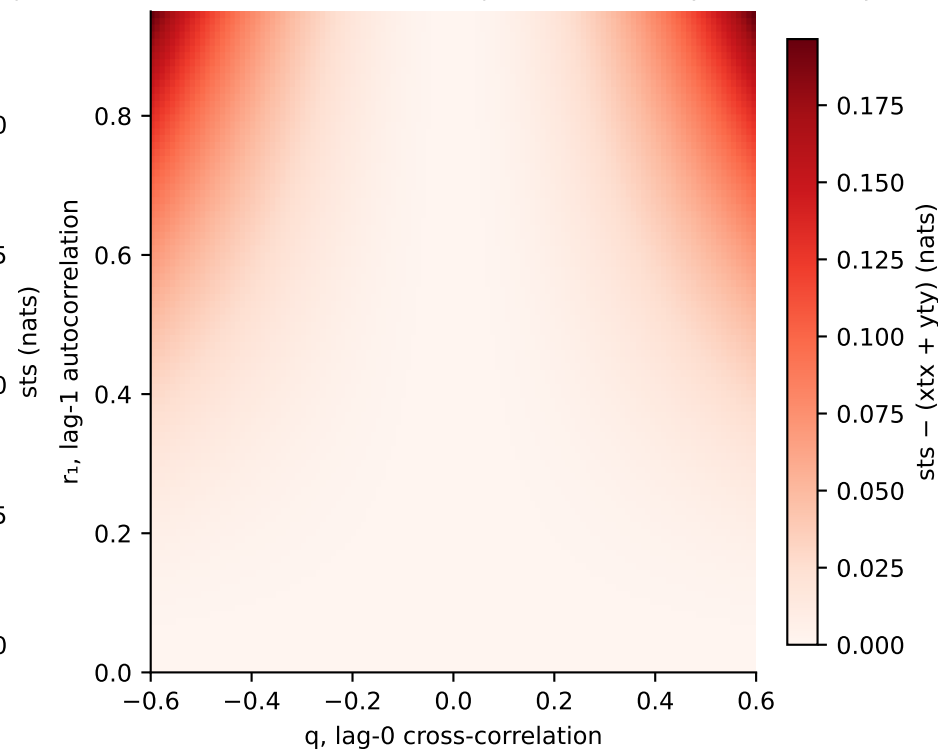
b the excess of sts over self-prediction (= rtr, symmetric family)
