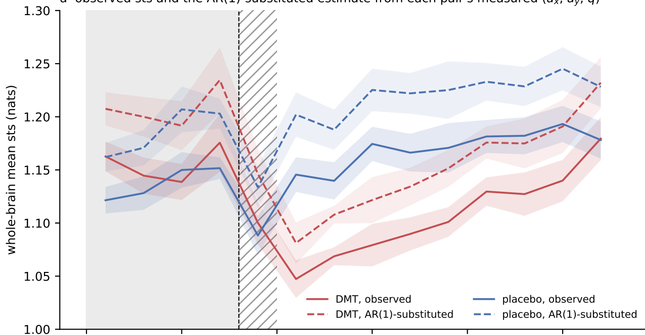
a observed sts and the AR(1)-substituted estimate from each pair's measured ( a_x, a_y, q )
