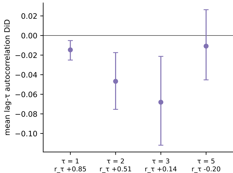
b the lag- \tau autocorrelation contrast
