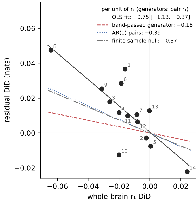
c the residual against the r_1 contrast
