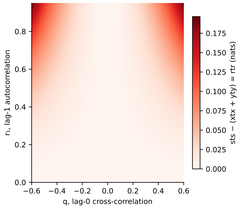
b the excess of sts over self-prediction (= rtr)
