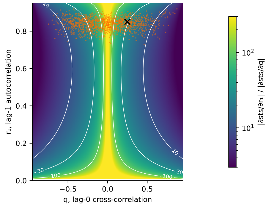
c which input sts responds to (no ratio = 1 boundary exists)
