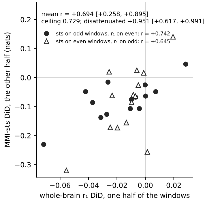
b the cross-half relation
