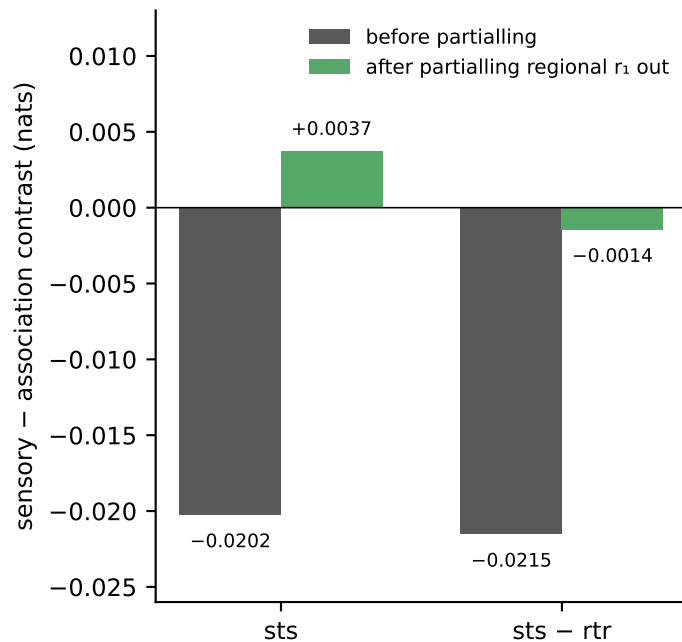
b the sensory-association contrast of the group map
