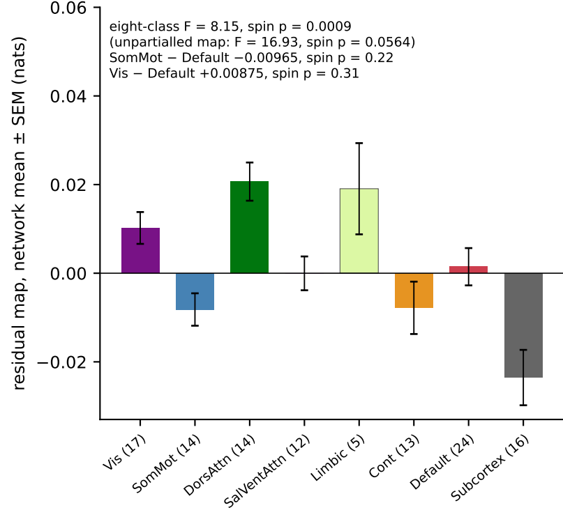
c the residual map's network means
