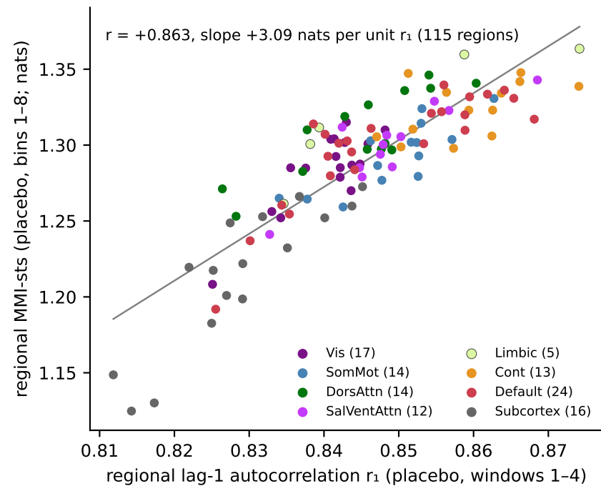
a regional synergy against regional autocorrelation
