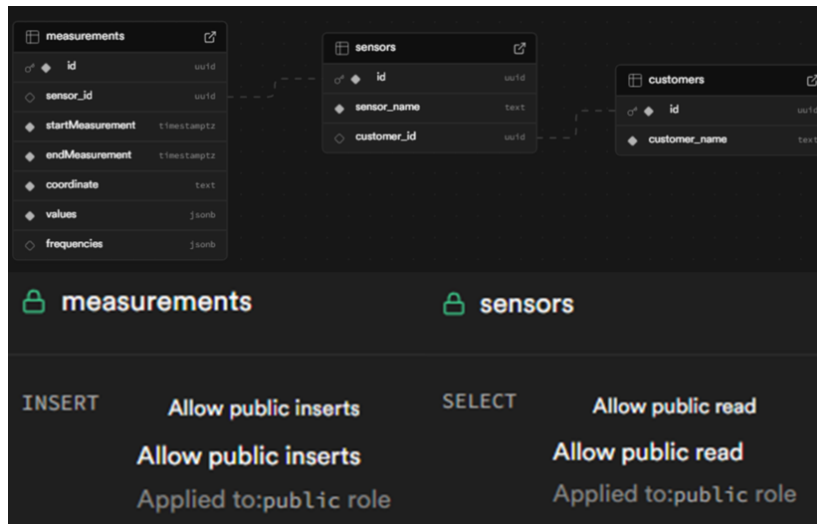
Figure 4.4: Entity-relationship schema of the Supabase database.
