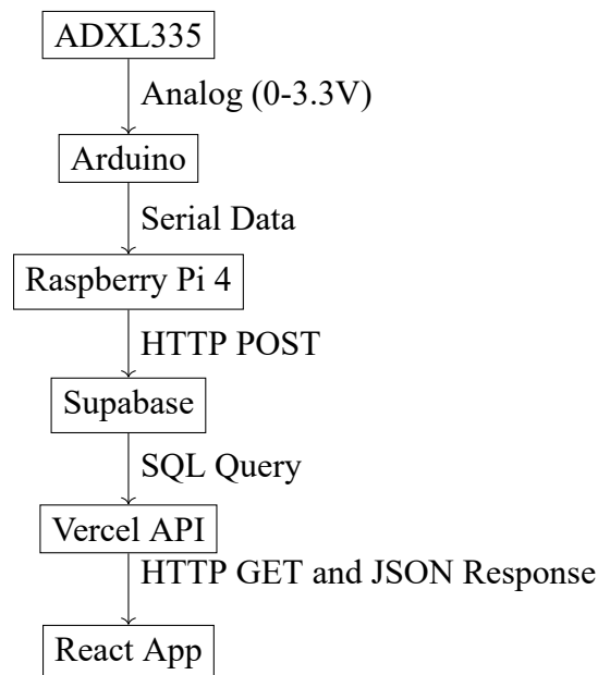
Figure 4.3: Complete system architecture and data flow from physical sensor to web visualization dashboard
