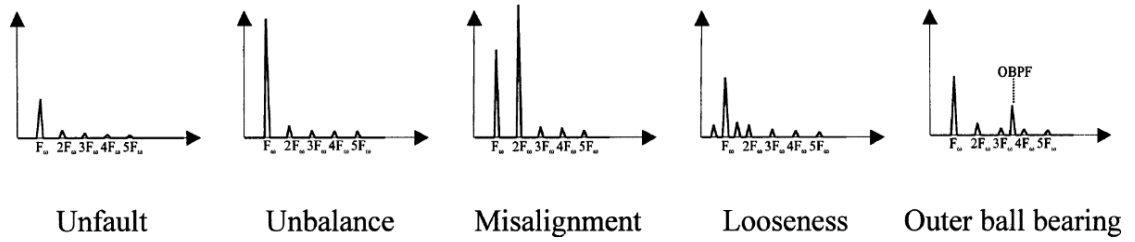
Figure 2.4: Fault and unfault spectrum graphs [2].
