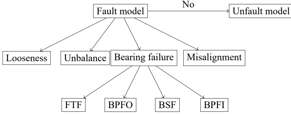
Figure 2.5: Fault tree analysis diagram showing the relationship between machine conditions and specific fault frequencies.
