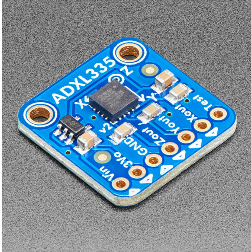
Figure 2.3: ADXL 335 accelerometer.
