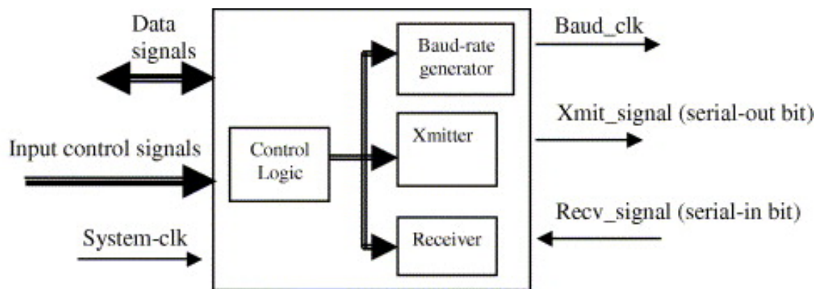
Figure 2.9: The UART block diagram. Source: [5].
