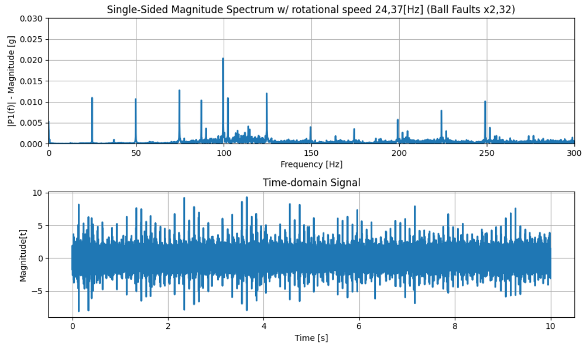
Figure .1: First bearing ball fault for rotational speed 24,37[Hz] [9].
