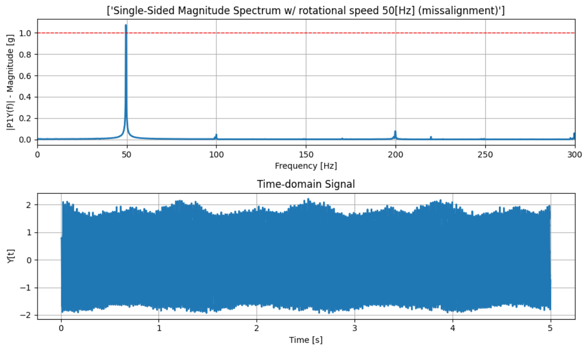
Figure .9: First motor misalignment fault at rotational speed 50[Hz] [10].
