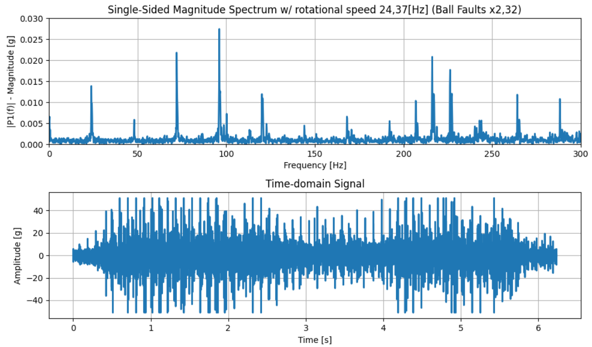
Figure .2: Second bearing ball fault for rotational speed 24,37[Hz] [9].
