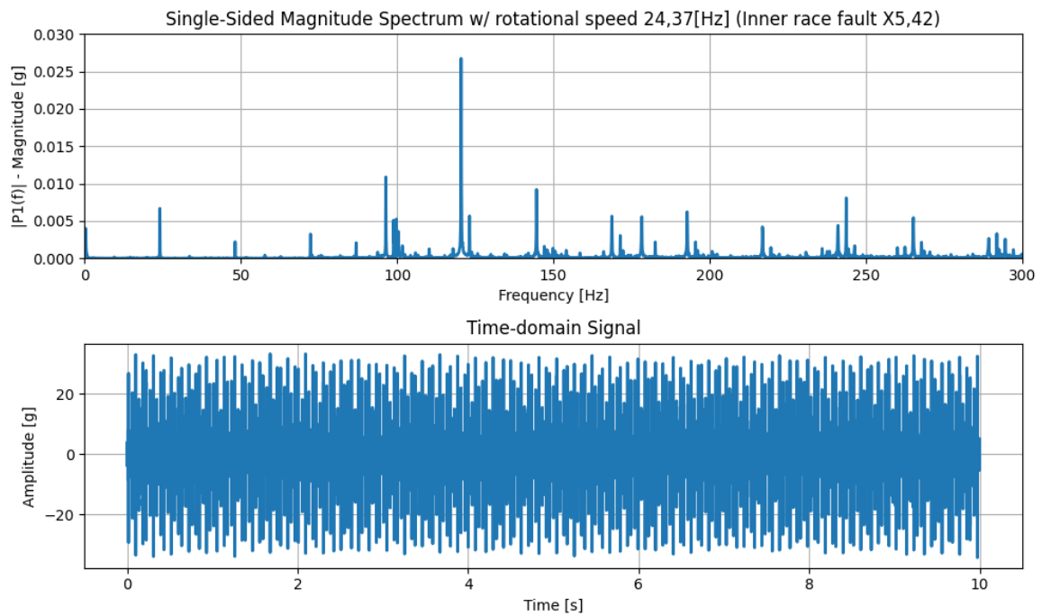
Figure .5: Second bearing inner racing fault for rotational speed 24,37[Hz] [9].
