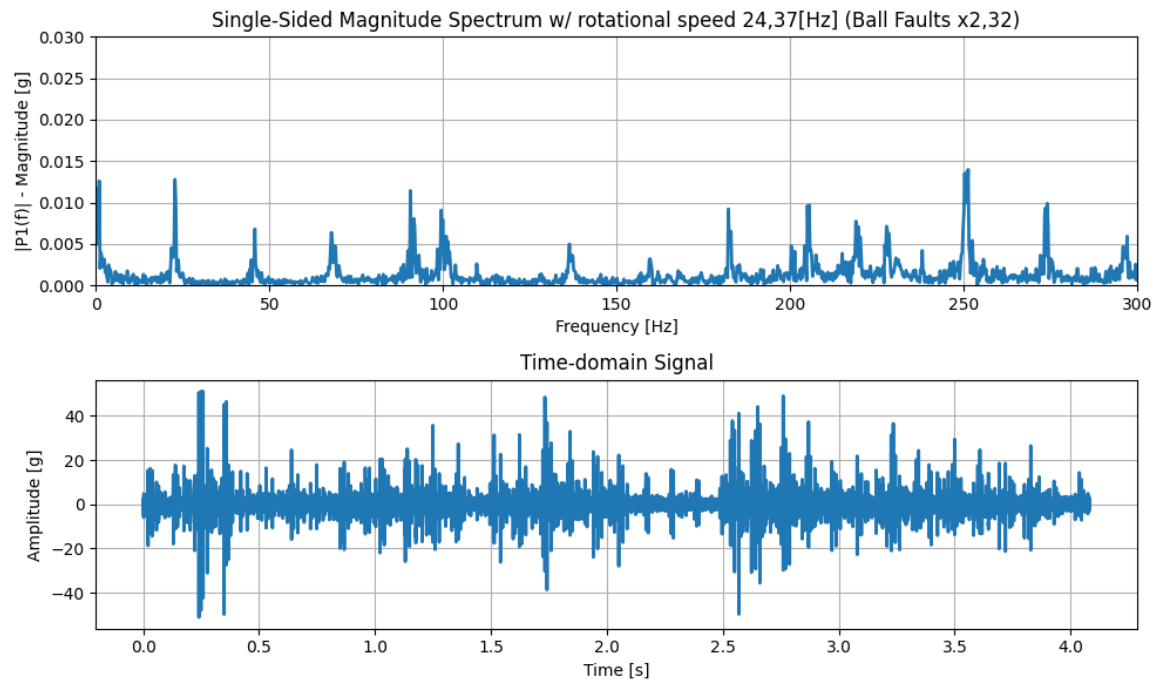
Figure .3: Third bearing ball fault for rotational speed 24,37[Hz] [9].
