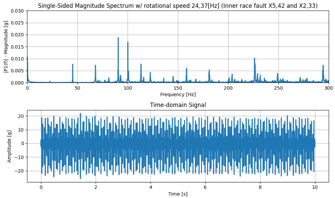
Figure .6: Third bearing inner racing fault for rotational speed 24,37[Hz] [9].
