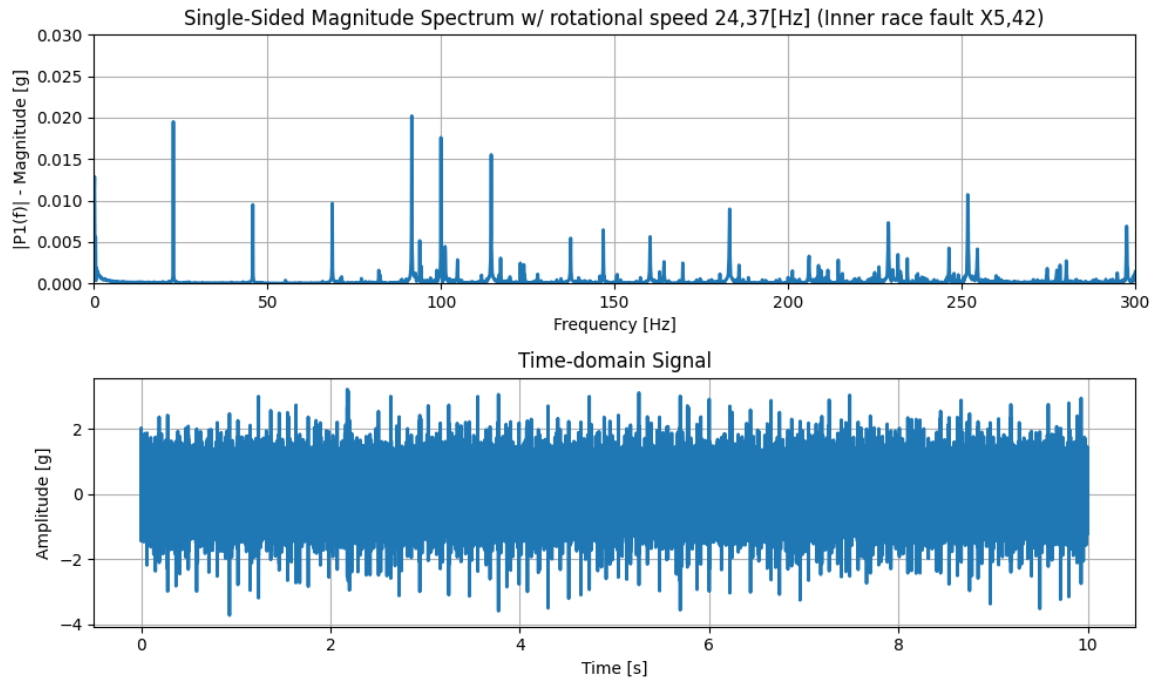
Figure .4: First bearing inner racing fault for rotational speed 24,37[Hz] [9].
