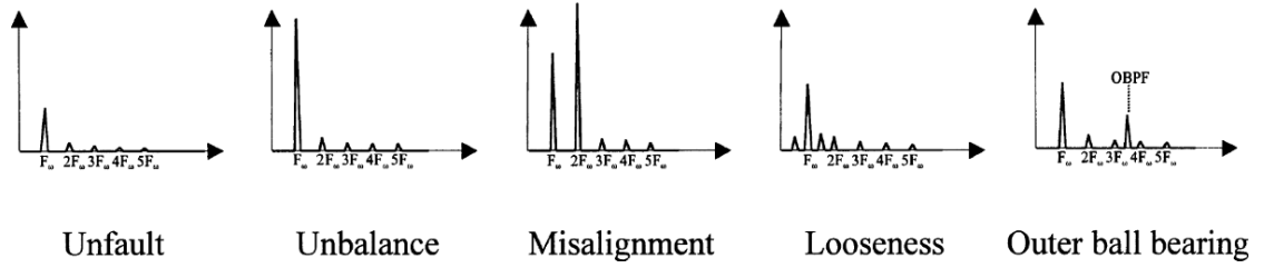
Figure 2.2: Fault and unfault spectrum graphs [2].
