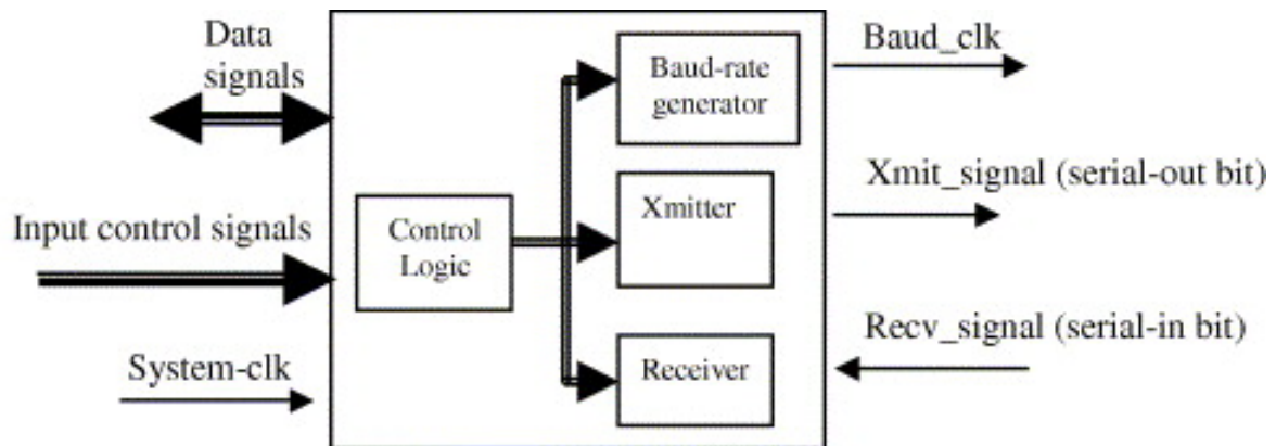
Figure 2.7: The UART block diagram. Source: [5].
