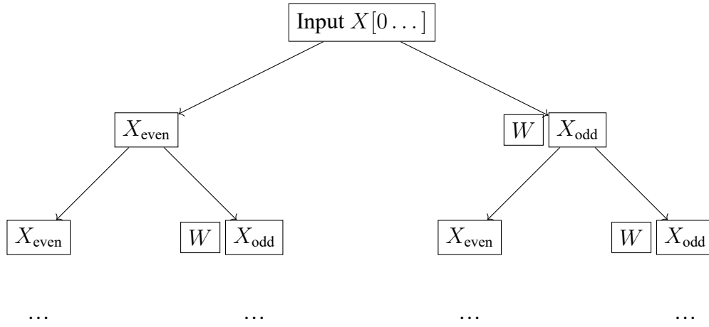
Figure 2.8: Recursive decomposition using even-odd splitting.
