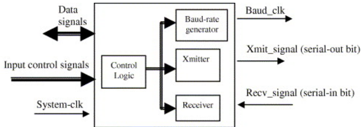
Figure 2.10: The UART block diagram. Source: [5].
