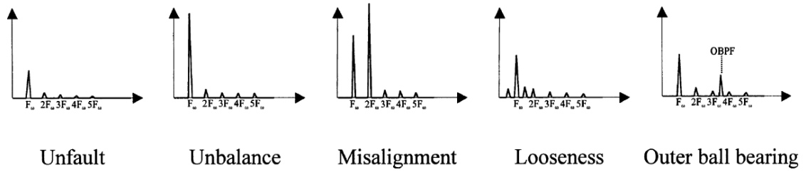
Figure 2.5: Fault and unfault spectrum graphs (source: [2]).
