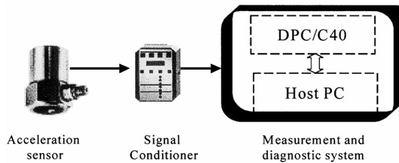
Figure 2.3: Block diagram of the designed station for vibration analysis (source: [2]).
