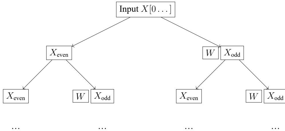
Figure 2.4: Recursive decomposition using even-odd splitting.
