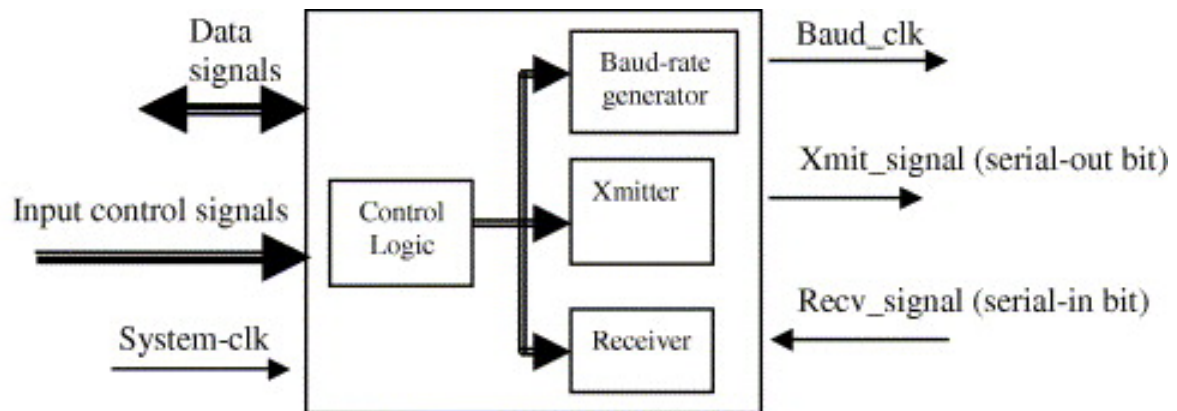
Figure 2.6: The UART block diagram. Source: [4].
