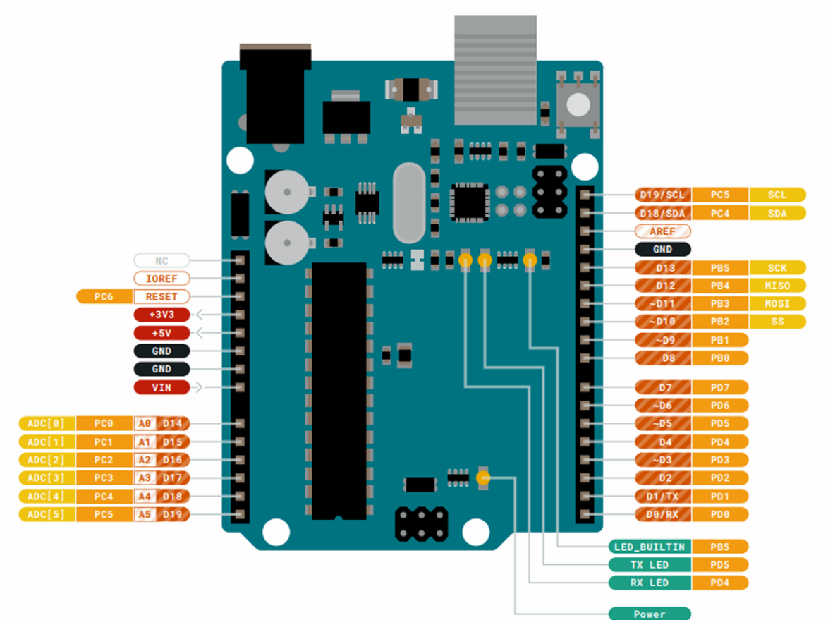
Figure 3.2: Arduino schematic pinout (refer to Tables 3.1 and 3.2 for details).
