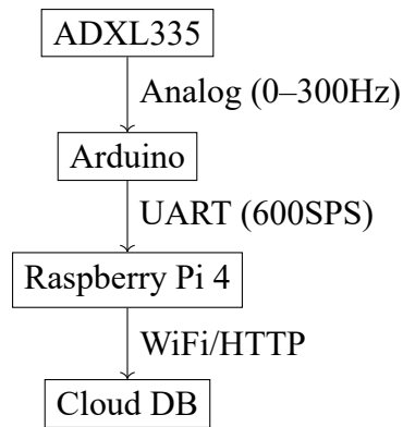
Figure 3.5: End-to-end data flow with protocols
