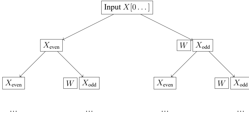
Figure 2.12: Recursive decomposition using even-odd splitting.
