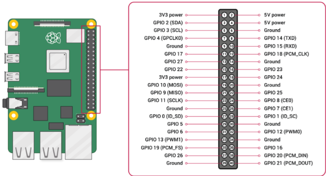
Figure 3.3: 40-PIN GPIO of Raspberry Pi 4 (source [23]).
