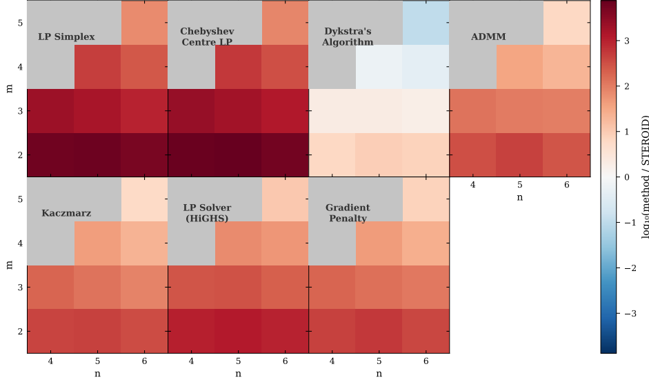
FIG. 4. Query speedup vs. STERIOD (log ratio; blue = faster than STERIOD).
