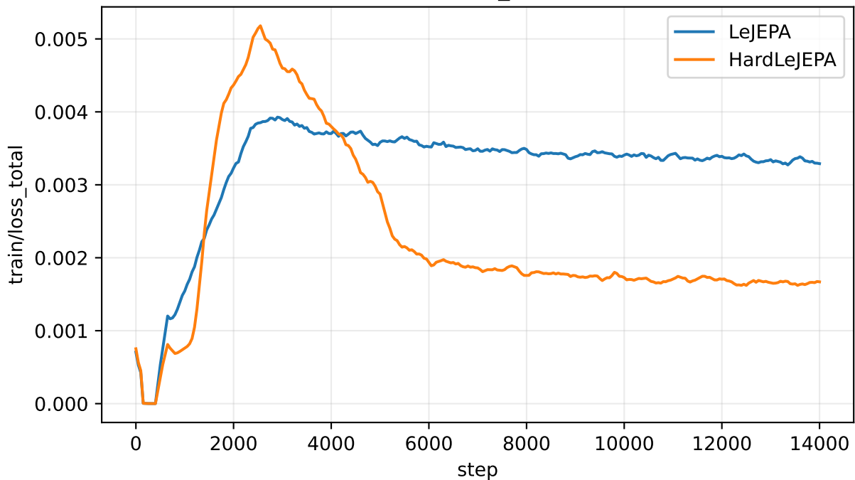
train/loss_total
