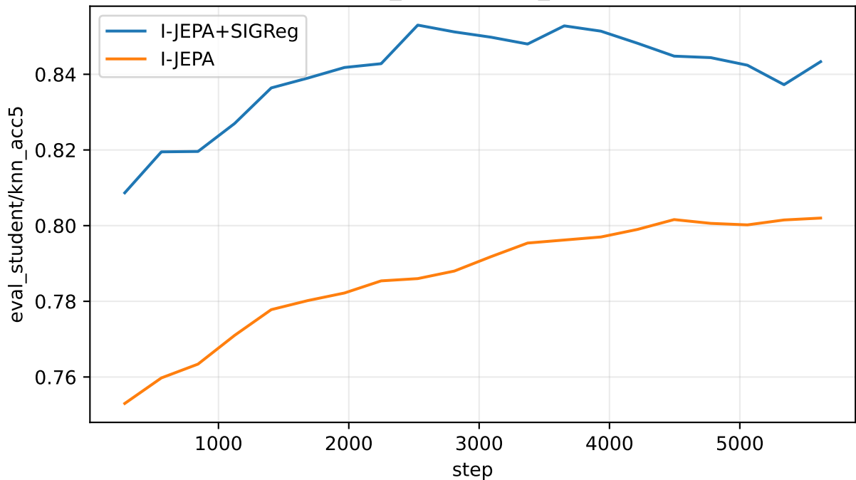
eval_student/knn_acc5
