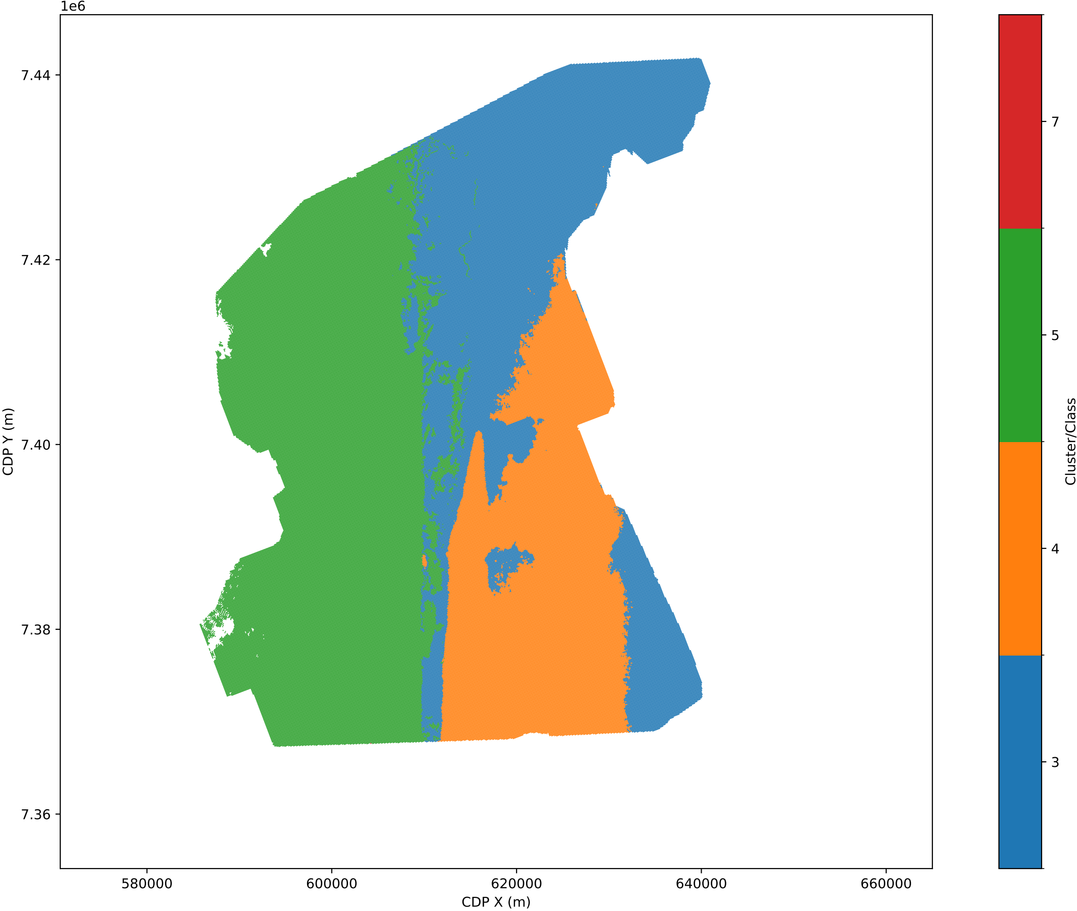
Reflecting horizon cluster map, ARI=0.496
