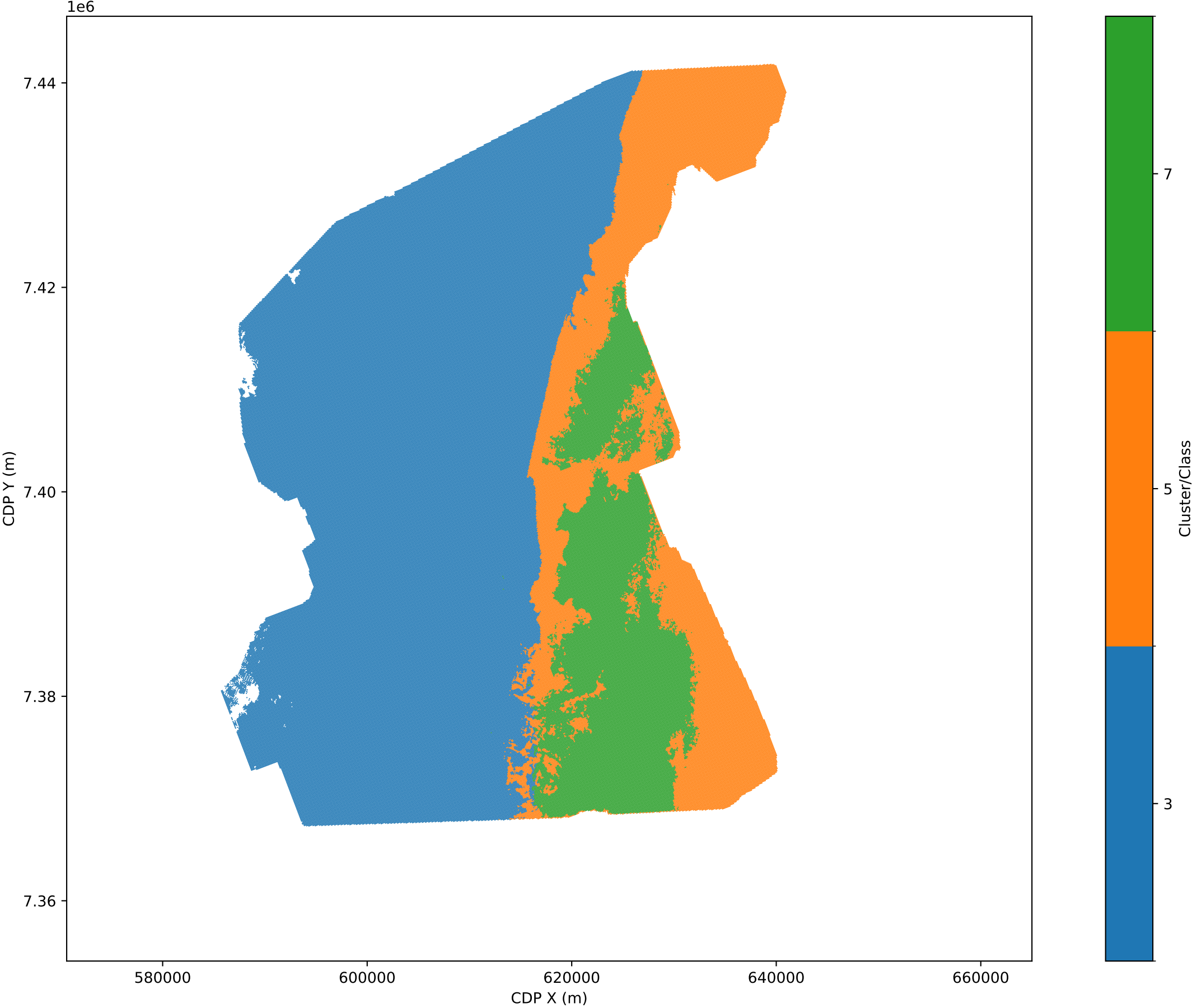
Reflecting horizon cluster map, ARI=0.612
