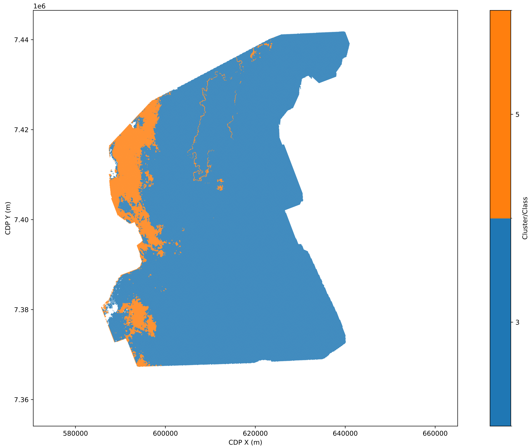
Reflecting horizon cluster map, ARI=-0.030
