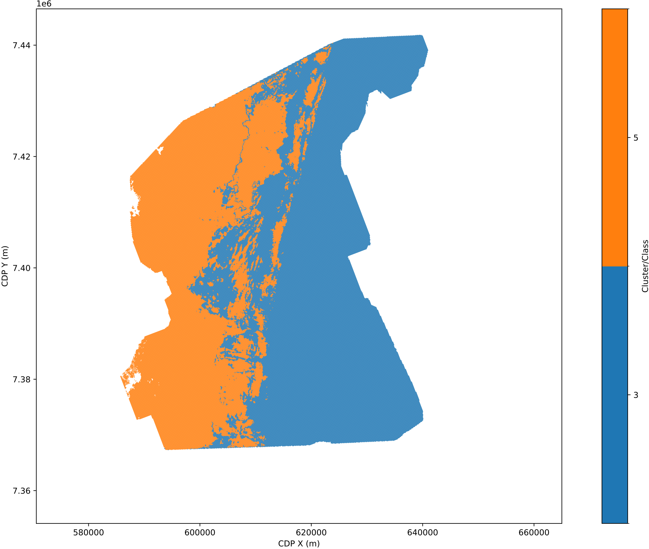
Reflecting horizon cluster map, ARI=0.444
