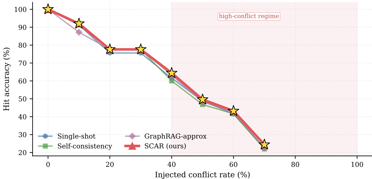
Robustness under source conflict (gold star = SCAR best-or-tied)
