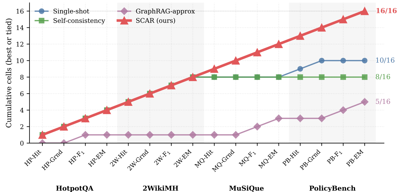
Cumulative best-or-tied count across the 16 FLAN-T5-Large cells
