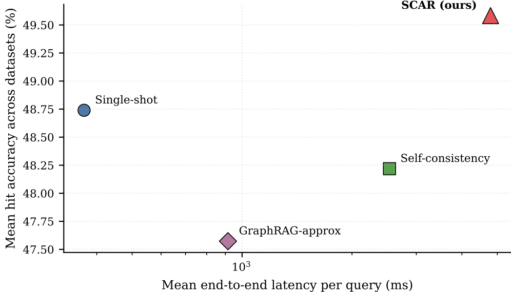
Accuracy-latency Pareto (FLAN-T5-Large)
