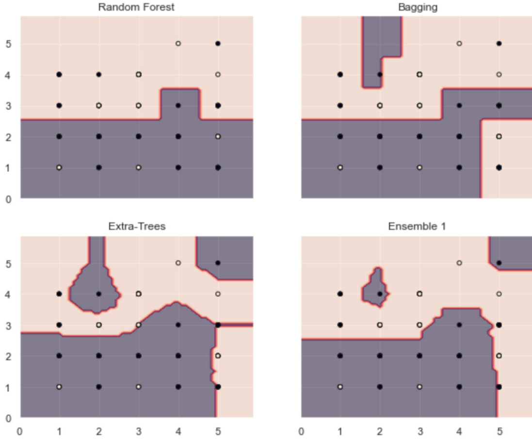
Fig. 8. Bagging Decision Boundaries.
