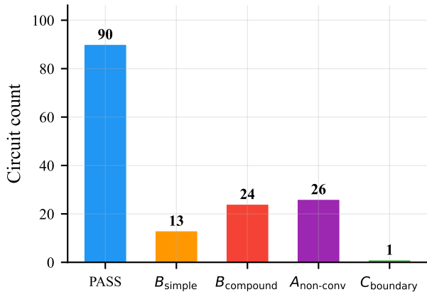
(a) Failure mode distribution ( n = 154 )
