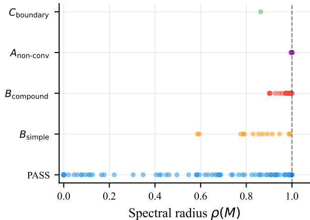
(b) \rho(M) by failure mode
