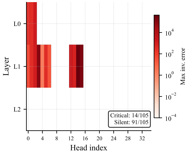
(a) T1 head ablation — max error (log scale; dark = critical)
