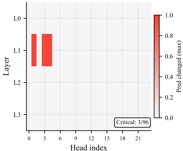
(b) T2 head ablation — output changed (red = ablation changes prediction)
