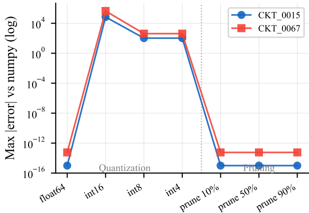
(a) T1: Quantization brittle, pruning robust
