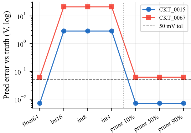
(b) T2: Quantization brittle, pruning robust
