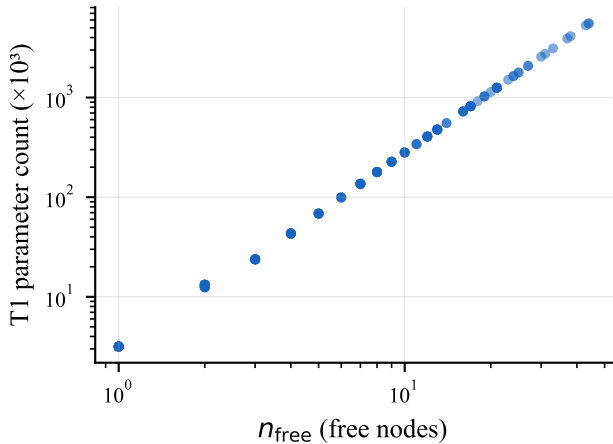
(a) T1 model size vs circuit size
