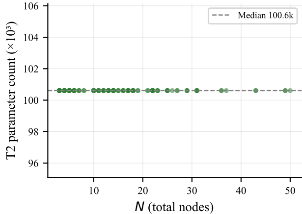
(b) T2 model size vs circuit size
