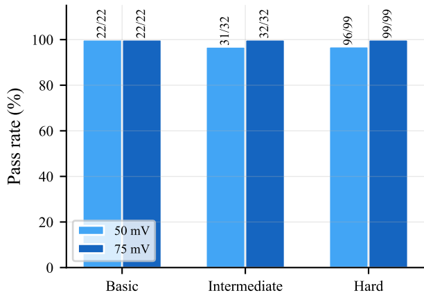
(b) Pass rate by complexity
