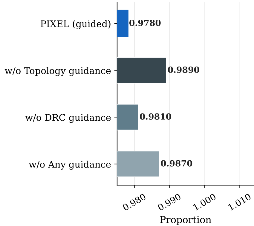
Connectivity Yield (post-processed)
