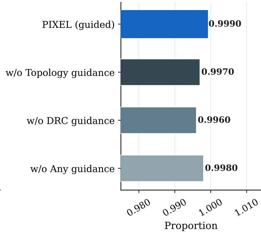
DRC Pass Rate (post-processed)
