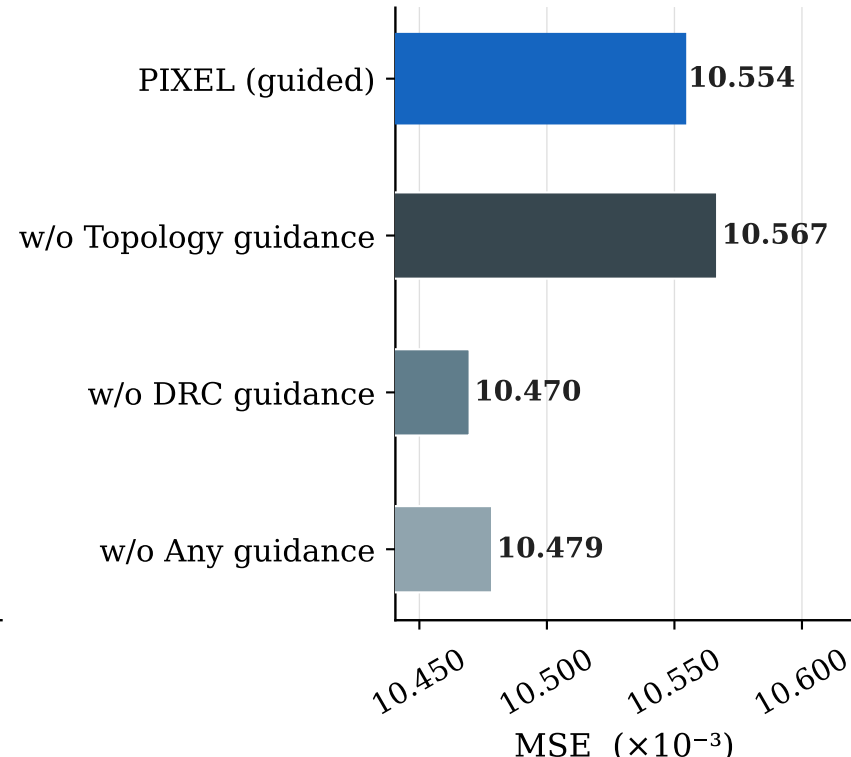
Surrogate S21 MSE ( \times 10^{-3} )
