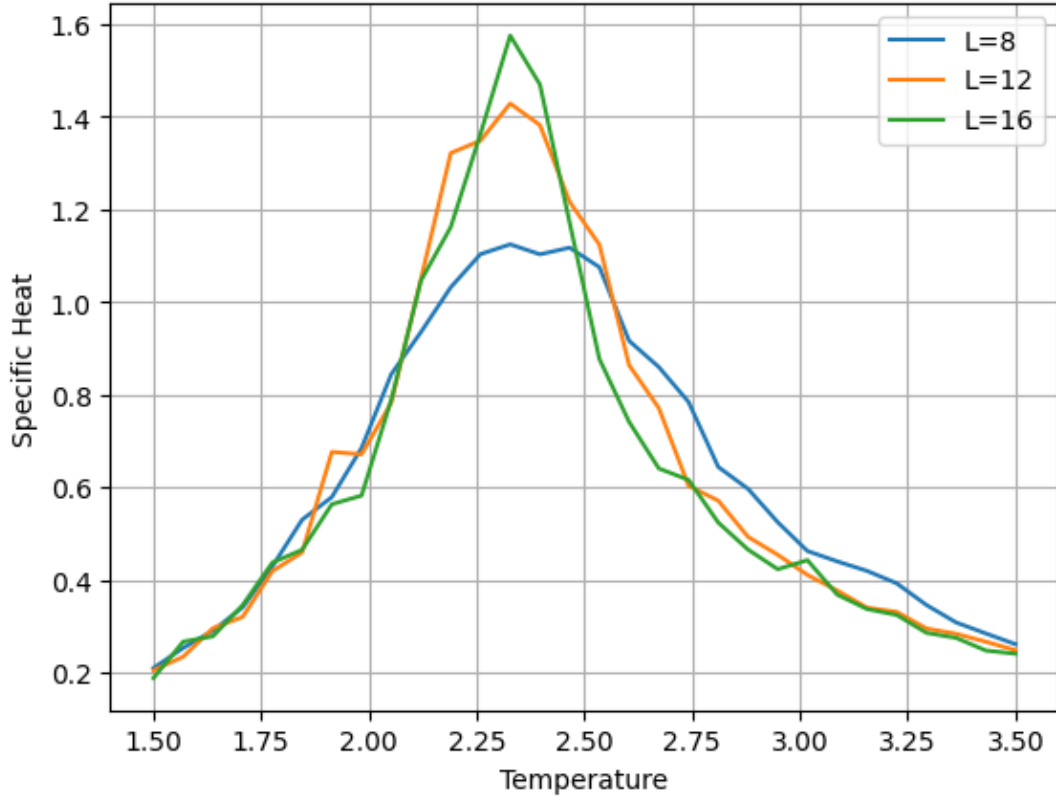
Figure 8: Specific Heat C_V vs Temperature. The peaks align near the theoretical critical temperature T_c \approx 2.269 .
