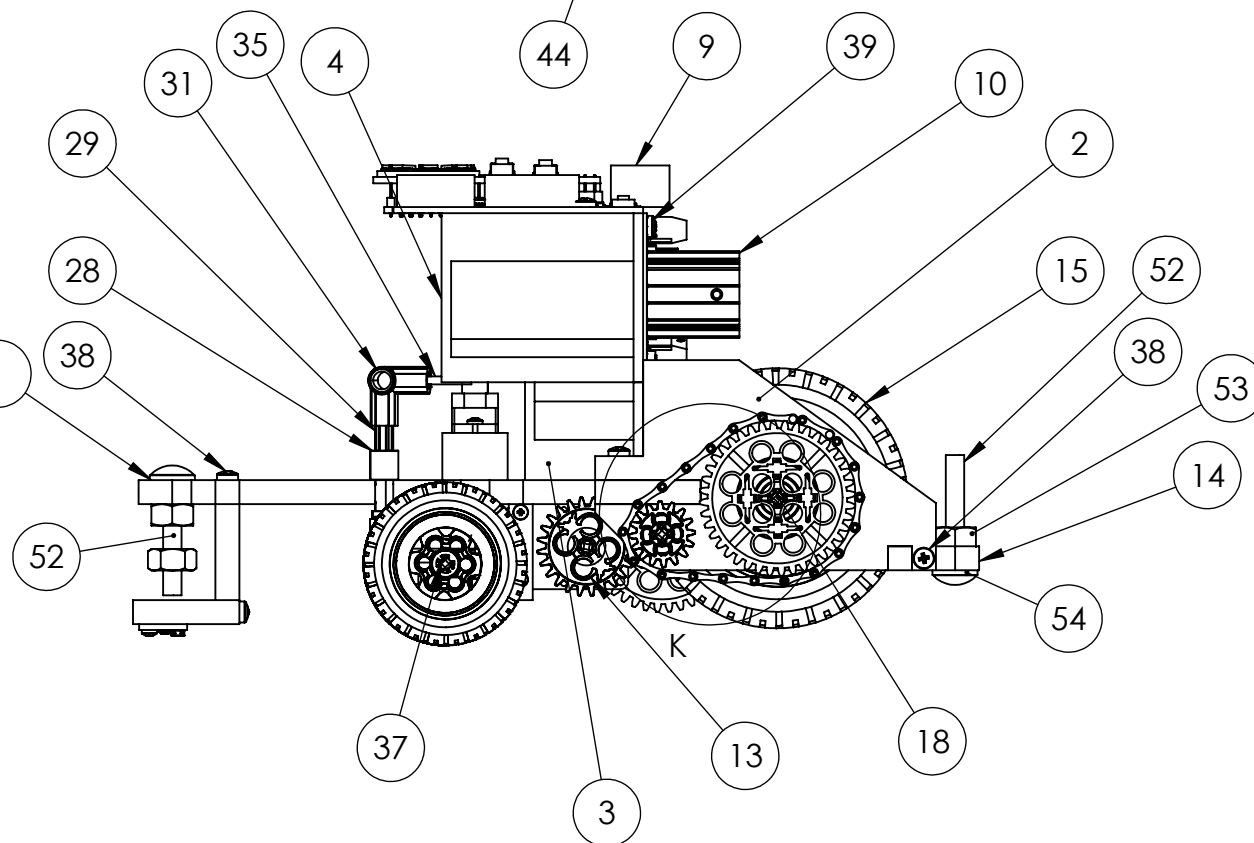
DETAILED E VIEW
