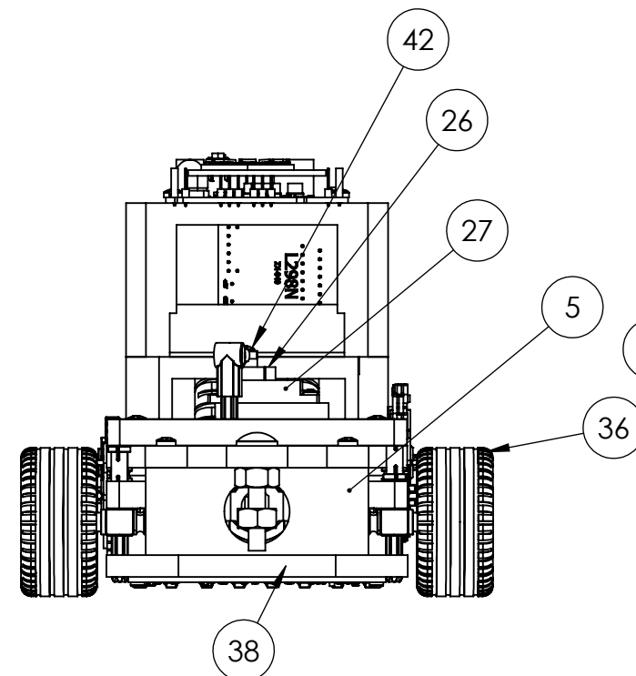
DETAILED K VIEW
