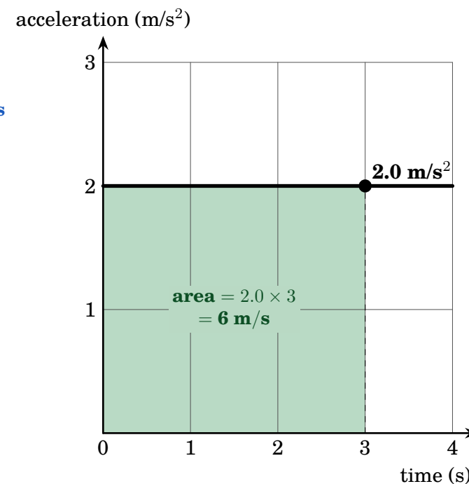
acceleration-time
