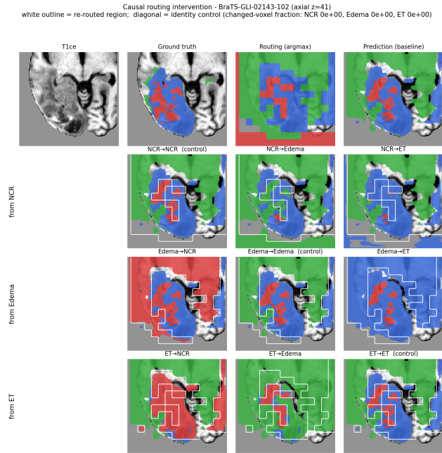
Figure 1. Causal intervention, rendered. Top: input, ground truth, routing argmax, baseline prediction. Grid: rows are the source concept, columns the target ; each cell is the segmentation after forcing every token the router assigned to the row concept through the column concept’s expert, with the re-routed region outlined in white. The diagonal is the identity control and is pixel-identical to the baseline (changed-voxel fraction 0 for all three), so the off-diagonal changes are attributable to re-routing alone.
