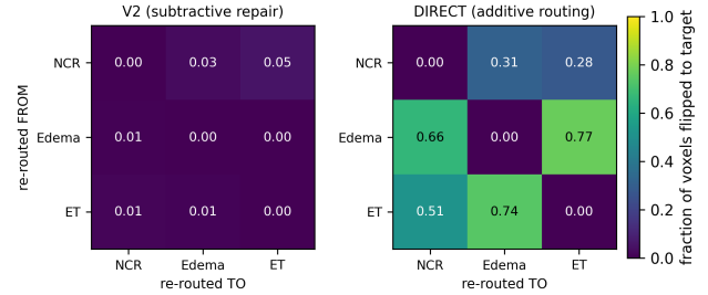
Figure 2. Causal control, V2 vs. DIRECT , on a shared colour scale. Rows are the source concept, columns the target; each cell is the fraction of re-routed voxels whose predicted label became the target. Subtractive repair leaves the matrix uniformly dark; additive routing does not. Diagonals are the identity control and are exactly zero in both.
