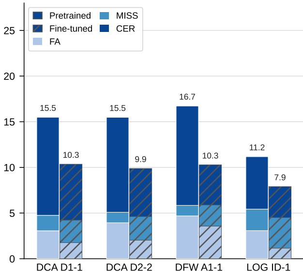
Diarization Error Rate (%)
