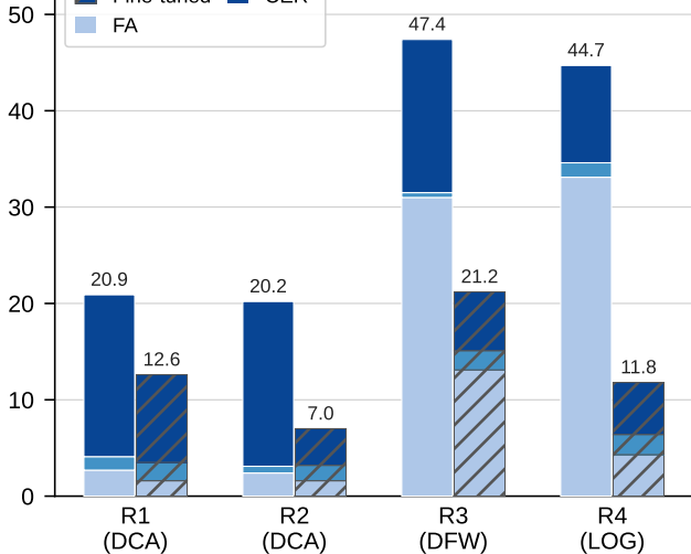
Diarization Error Rate (%)
