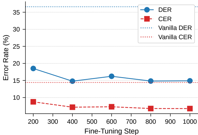
Evaluation DER and CER
