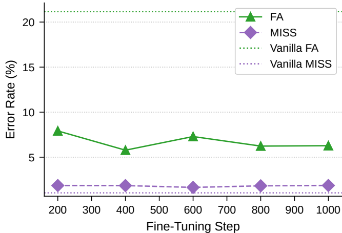
Evaluation FA and MISS
