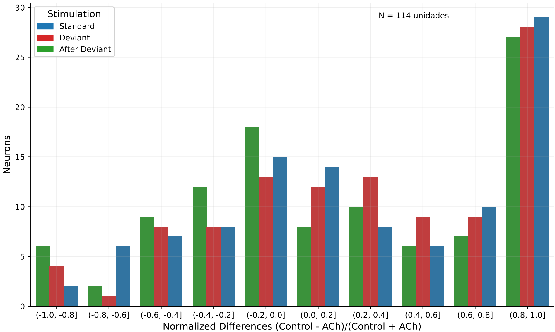
Distribution of Normalized Differences in Firing Rate by Stimulation Type
