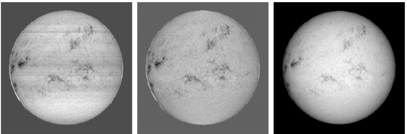
From left to right: single Helium ray image generated by INTI, image with Helium image enhancement, image with enhancement and combination with continuum image.
