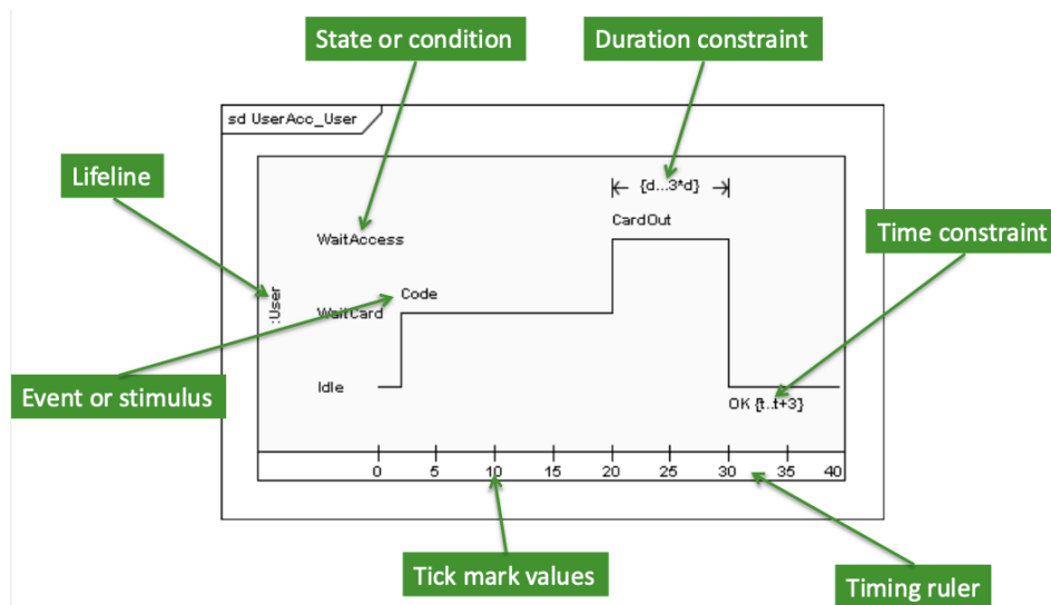
Figure 13.15: A Timing Diagram showing state changes along a time ruler.
