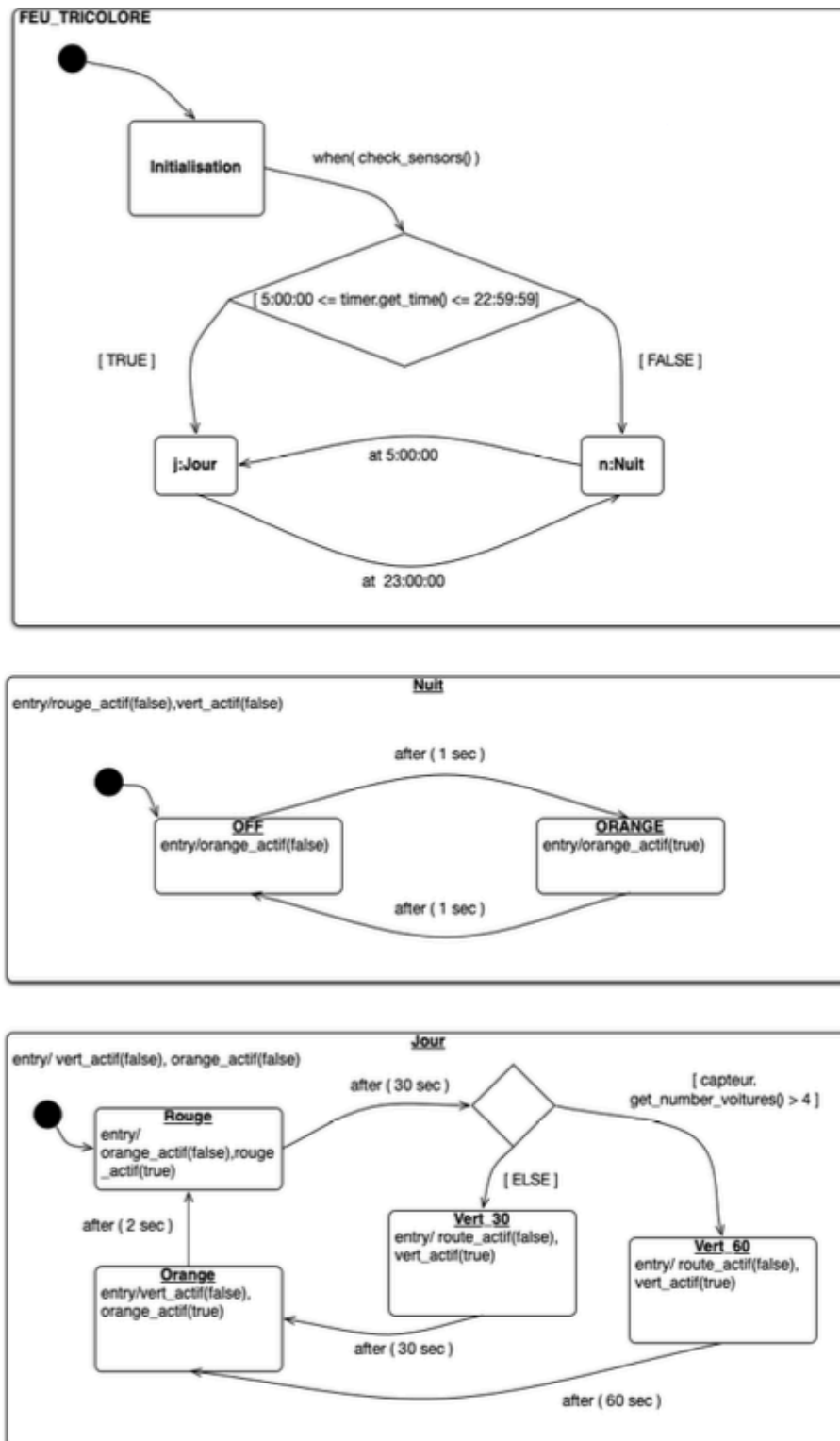
Figure 10.2: State Machine Diagram for the Traffic Light System.
