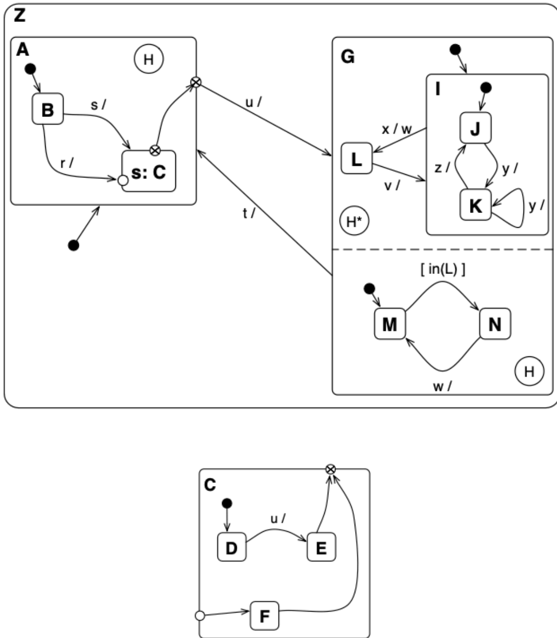
Figure 9.4: State Machine and Submachine for Exercise 2.
