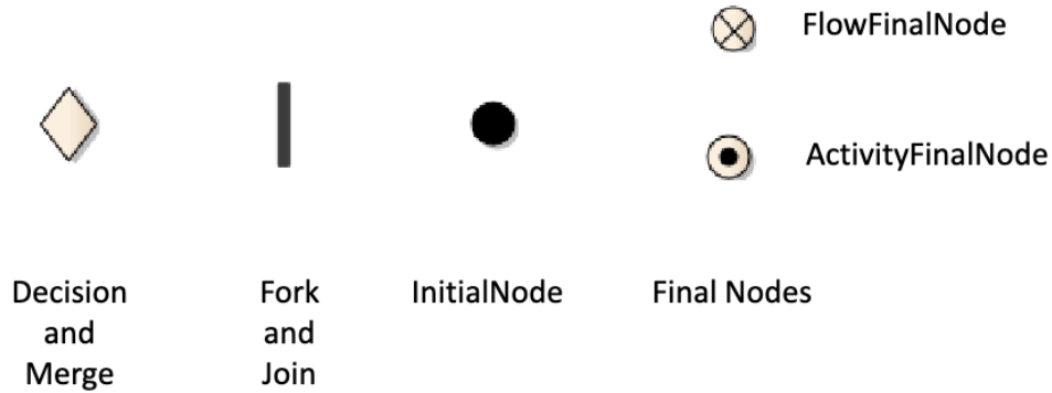
Figure 11.3: Various UML Control Nodes: Initial, Final (Activity/Flow), Decision/Merge, Fork/Join.
