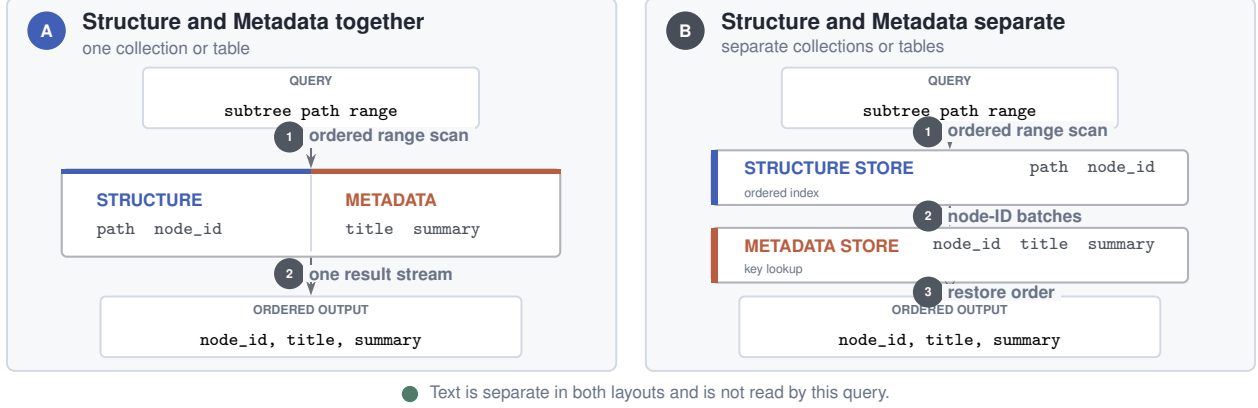
Figure 1: The two layouts used for get_subtree . Left: Structure and Metadata are together and are read by one ordered range scan. Right: Structure and Metadata are separate, so the Structure scan returns node IDs, Metadata is fetched in batches, and the records are restored to Structure order. Both paths return the same ordered rows. The arrows show query steps, not stored pointers. Text is separate in both layouts and is not read by this operation.
