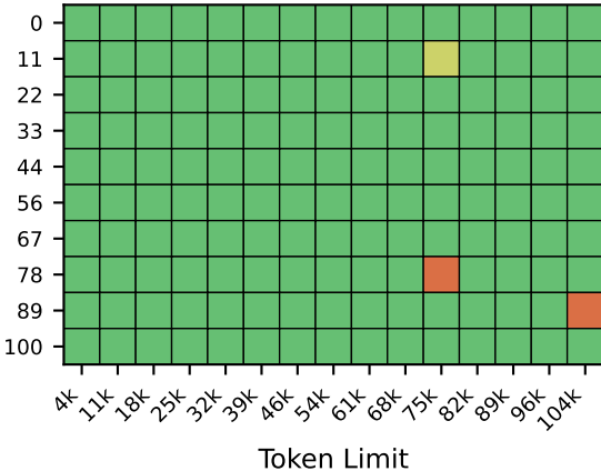
Full-Precision Score: 0.987
