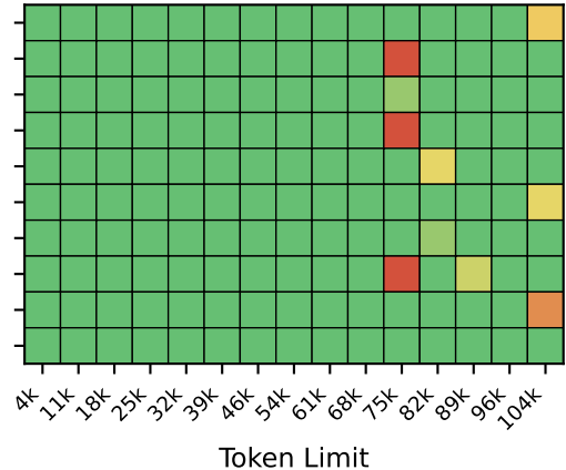
TurboQuant 3.5-bit Score: 0.962
