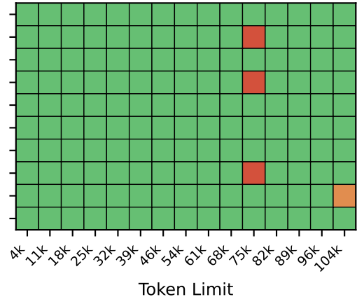
RaBitQ 3.5-bit Score: 0.977
