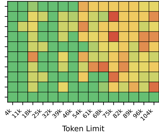
TurboQuant 2.5-bit Score: 0.709
