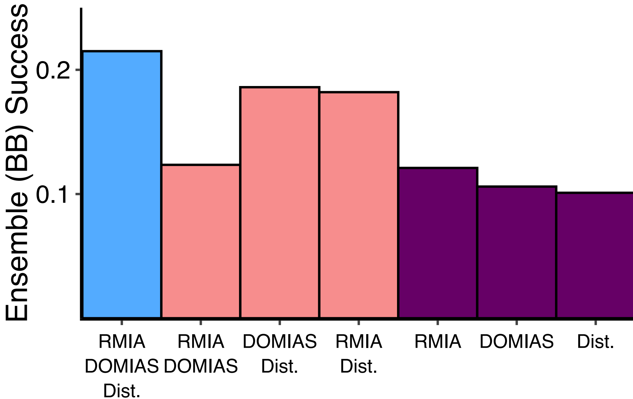
Berka Ensemble Ablations
