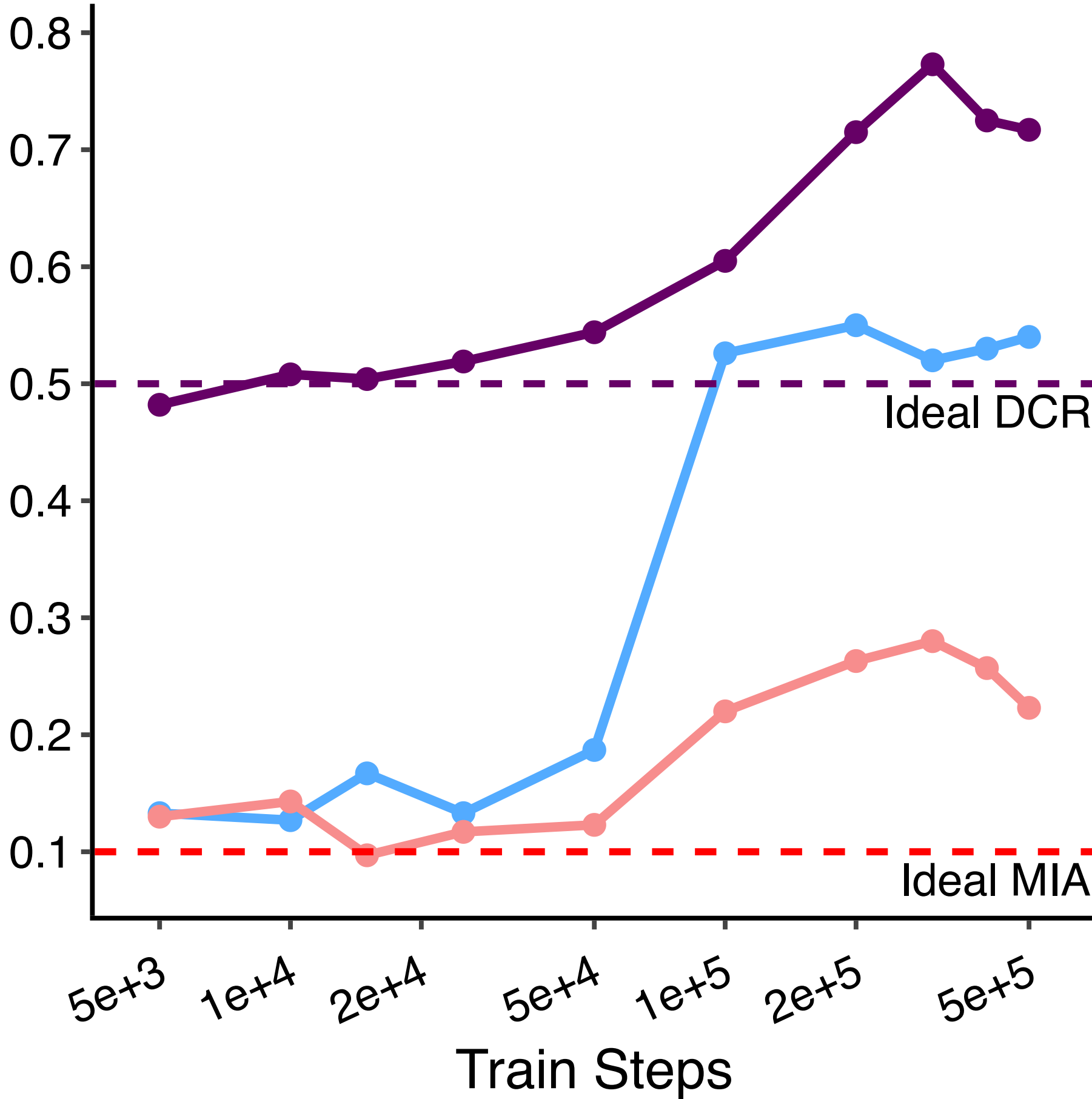
Metric Score
