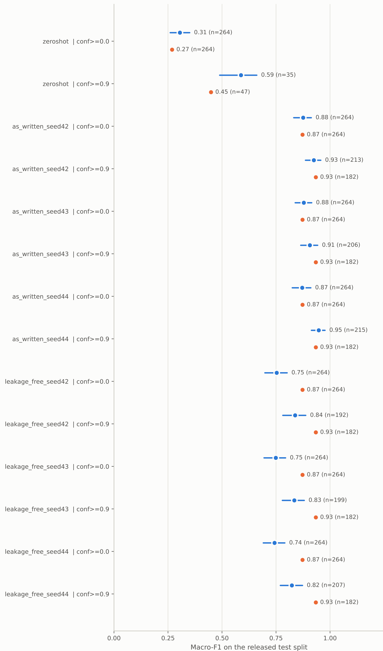
Faulborn stance classifier: reconstruction vs reported macro-F1
