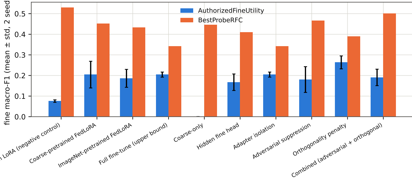
Phase 1+2 fair baselines — HIERARCHICAL FIXTURE (real learnable signal, still synthetic)
