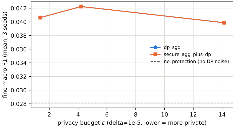
Phase 4 privacy-utility Pareto — SYNTHETIC TIER (pipeline validation only)
