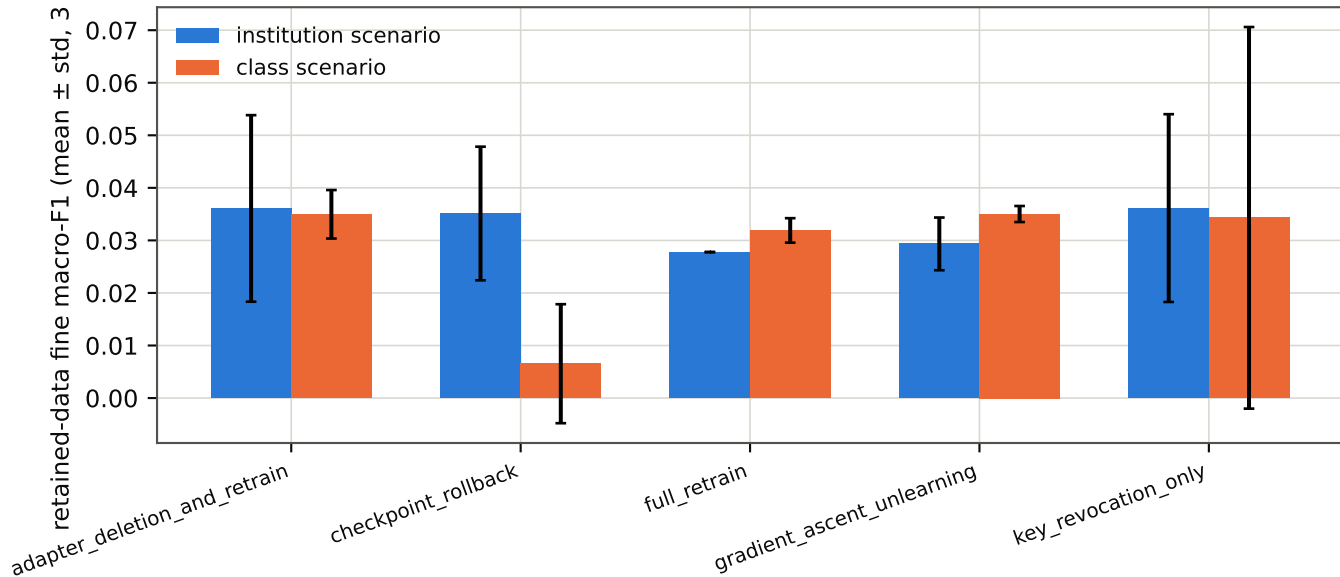
Phase 5 unlearning vs. retraining — SYNTHETIC TIER (pipeline validation only)
